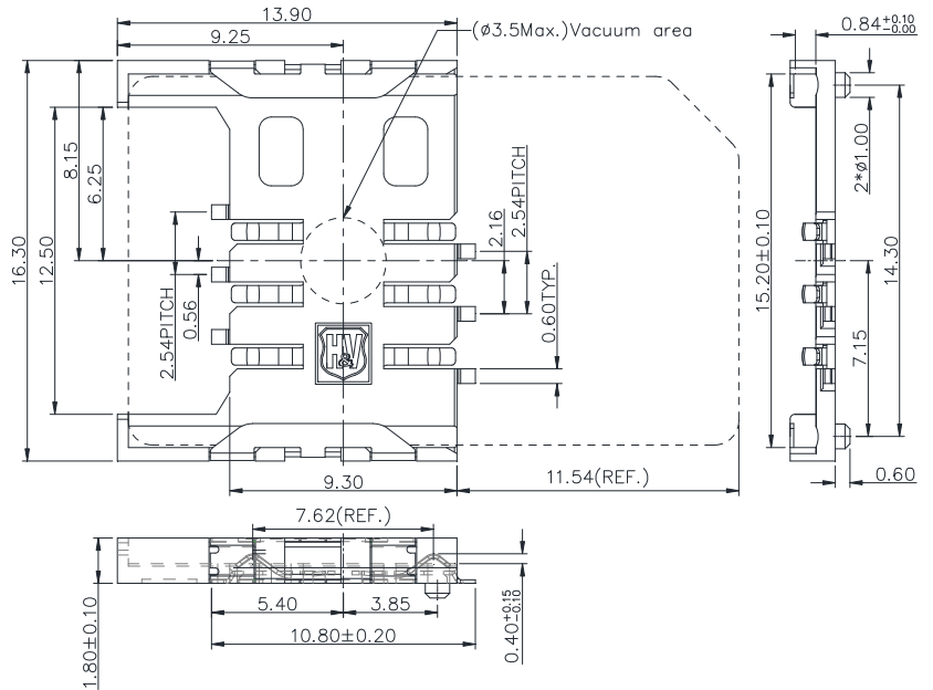
Unit: mm; Tolerances: ±0.15 mm Mechanical outline dimension
