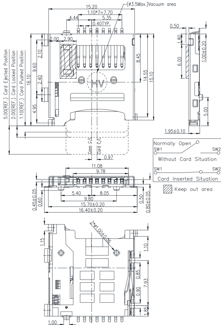
Unit: mm; Tolerances: ±0.15 mm Mechanical outline dimension
